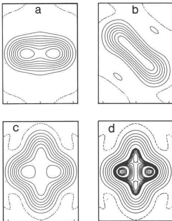
FIGURE 1. Difference-Fourier sections for fluor-cannilloite calculated through the central A2/m site with the A cation removed from the structural model (the contour interval is 1 \text{ e}/\text{\AA}^3 ): (a) (100) section at x = 0 ; (b) (010) section at y = 1/2 ; (c) section through the electron-density maxima on the twofold axis and in the mirror plane, parallel to (\bar{2}01) ; (d) the (\bar{2}01) section with 0.1 \text{ e}/\text{\AA}^3 contouring above 6 \text{ e}/\text{\AA}^3 .
