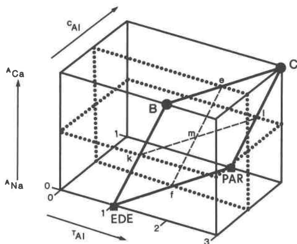
FIGURE 3. ACT compositional diagram for A-site-full calcic fluor-amphiboles. The A axis shows the Na = Ca substitution, the C axis shows the M^{2+} = M^{3+} substitution (written as {}^C\text{Al} ), and the T axis shows the Si = Al substitution (written as {}^T\text{Al} ). Compositions marked are as follows: EDE = \text{NaCa}_2\text{Mg}_5(\text{Si}_7\text{Al})\text{O}_{22}\text{F}_2 , PAR = \text{NaCa}_2(\text{Mg}_4\text{Al})(\text{Si}_6\text{Al}_2)\text{O}_{22}\text{F}_2 , B = \text{CaCa}_2\text{Mg}_5(\text{Si}_6\text{Al}_2)\text{O}_{22}\text{F}_2 , C = \text{CaCa}_2(\text{Mg}_4\text{Al})(\text{Si}_5\text{Al}_3)\text{O}_{22}\text{F}_2 .
