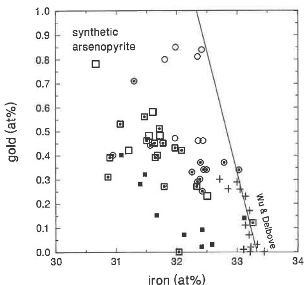
FIGURE 4. Variation of Au with Fe in euhedral grains of synthetic arsenopyrite. Open symbols are zones of light BSE contrast (cf. Fig. 2a), centered symbols are zones of medium contrast, and solid symbols are zones of dark contrast; squares are SA42 (400 °C, 57 d), circles are SA41 (400 °C, 57 d), crosses are data of Wu and Delbove (1989), line is substitution \text{Fe} = \text{Au} ; all data are calculated to the formula (\text{Fe}, \text{Au}, \square)\text{As}_{1 \pm x}\text{S}_{1 \pm x} .
