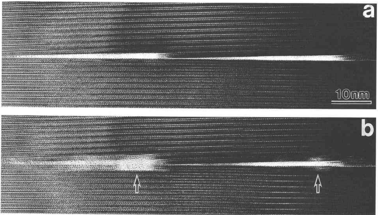
FIGURE 5. (a) Magnified image of a LAGB observed from (100). (b) Image of the same area after beam radiation for about 20 s. The chlorite layers on both sides of the boundary are starting to be vitrified as indicated by arrows. The structure in the chlorite layer can be distinguished in the thinner area (left side).
