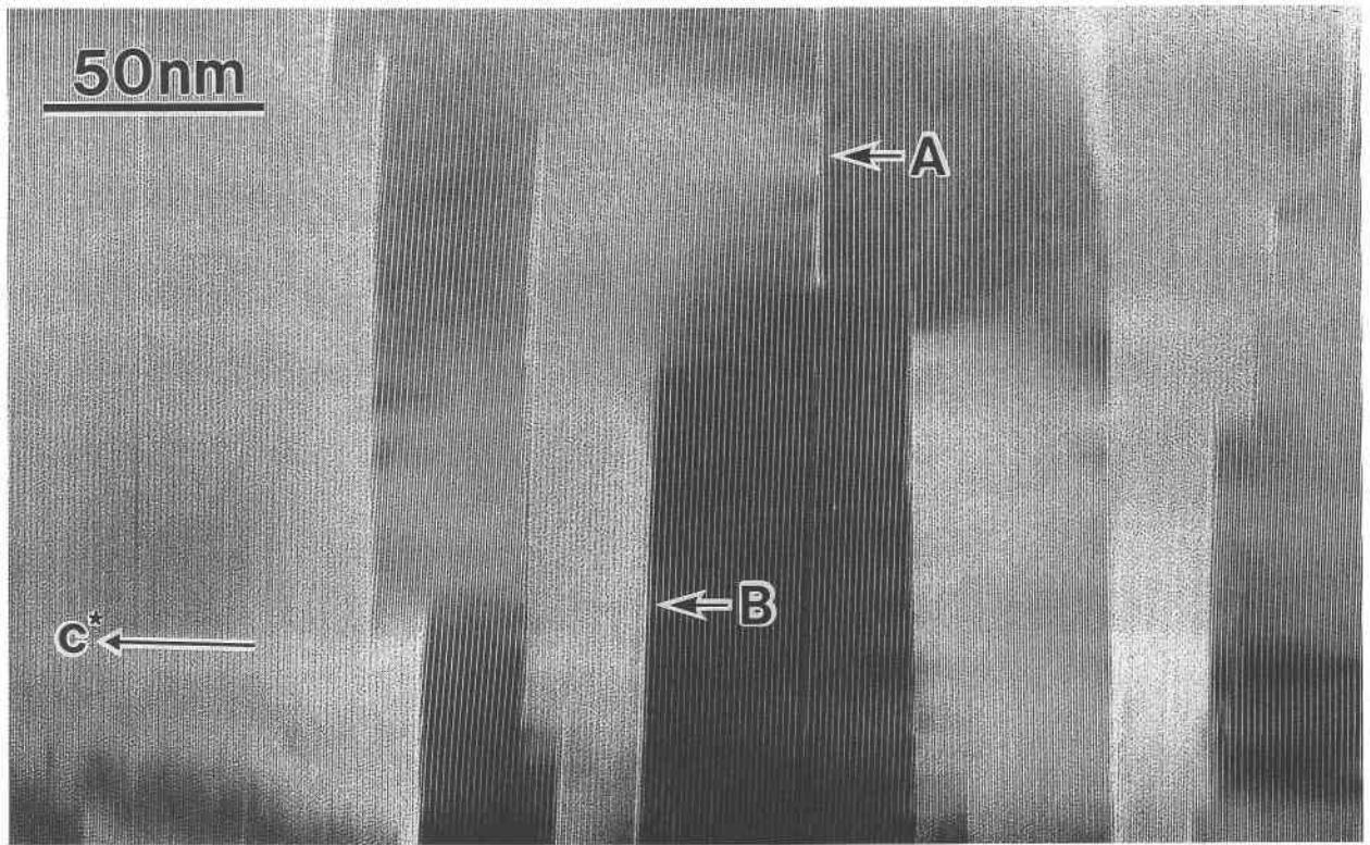
FIGURE 1. HRTEM image of chlorite from altered granite observed approximately along \langle 010 \rangle . Planar defects are observed commonly as indicated by the arrows A and B. At defect A the lattice fringes are inclined to each other whereas at defect B (001) fringes are almost parallel on both sides of the defect. Some planar defects are initiated or terminated in the grain.
