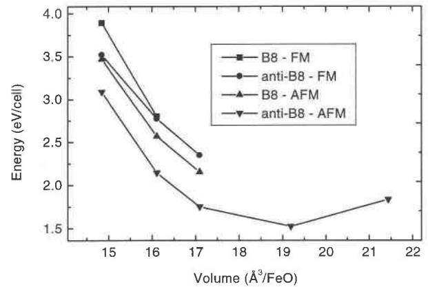
FIGURE 4. Total energies per cell (4 atoms) for B8 and anti-B8 with ferromagnetic (FM) and anti-ferromagnetic (AFM) ordering computed using the LAPW method within GGA.
