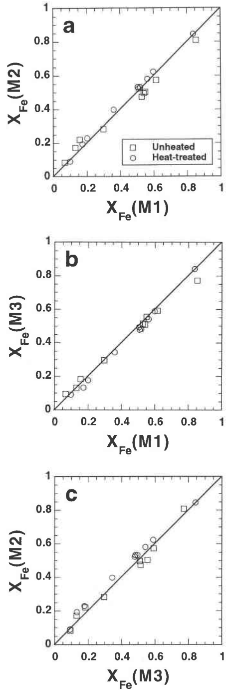
FIGURE 5. Roozeboom plots of M1, M2, and M3 site preference in the actinolite series, this work, assuming \text{Fe}^{3+} is located on M1 and M2 (see text).
