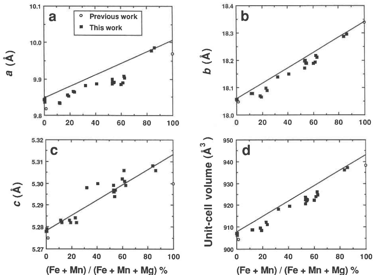
FIGURE 6. Cell dimensions as a function of macroscopic (\text{Fe} + \text{Mn})/(\text{Fe} + \text{Mn} + \text{Mg})\% . Filled squares = actinolite and ferroactinolite (this work) and tremolite (Yang and Evans 1996); circles = natural tremolite of Papike et al. (1969) and synthetic ferroactinolite of Ernst (1966). Straight line connects inferred dimensions of end-members tremolite and ferroactinolite (see text).
