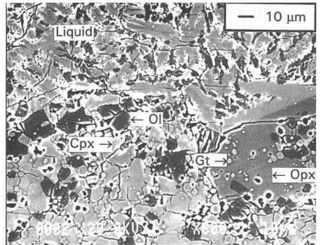
Mix 31 T = 2020 °C P = 10 GPa time = 7 min
