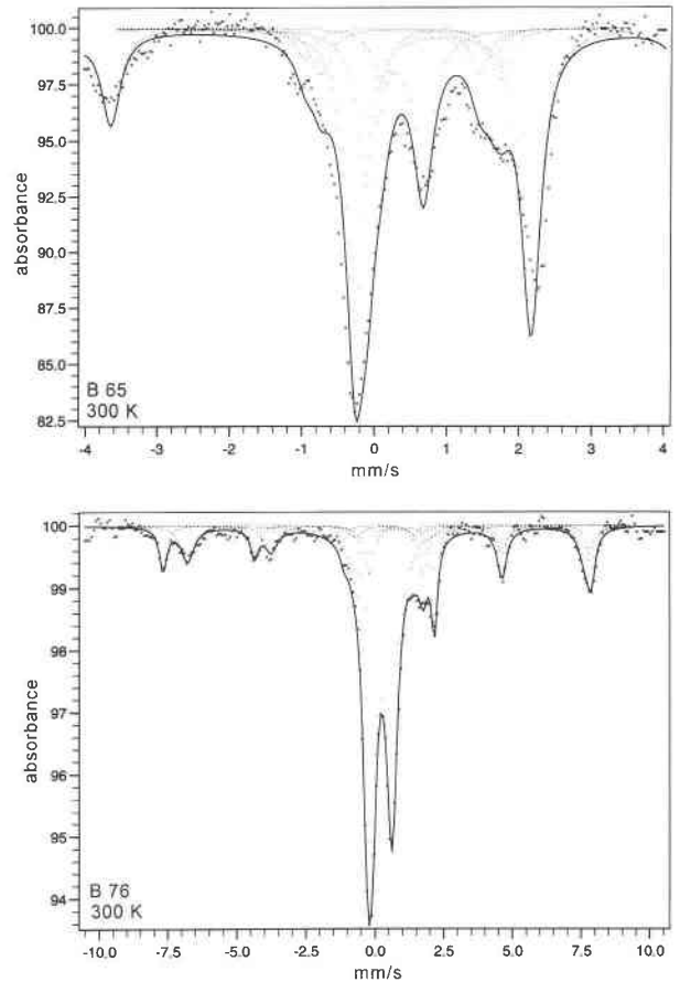
FIGURE 8. Mössbauer spectra obtained at 300 K of tourmalines [B65 (top) at 600 °C and B76 (bottom) at 700 °C] synthesized at f_{O_2} conditions of the HM solid buffer. The two spectra reveal the presence of two different Fe-oxide phases identified on the basis of MS and XRD as hematite and magnetite.
