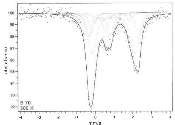
FIGURE 9. Mössbauer spectrum obtained at 300 K of tourmaline B70 synthesized at 600 °C at f_{O_2} conditions of the QFI solid buffer. Note the presence of two Fe^{3+} doublets; one can be attributed to Fe^{3+} in the Y (9b) site, but the attribution of the other remains doubtful.
