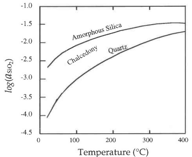
FIGURE 5. Calculated diagram showing the boundaries of aqueous silica activities for quartz and amorphous silica formation as a function of temperature at a pressure of 500 bars. The diagram was calculated using SUPCRT92 software and the database of Johnson et al. (1992). The region for chalcedony formation (between the saturation curves for quartz and amorphous silica) is constrained based on synthesized chalcedony that occurs only below 300 °C.
