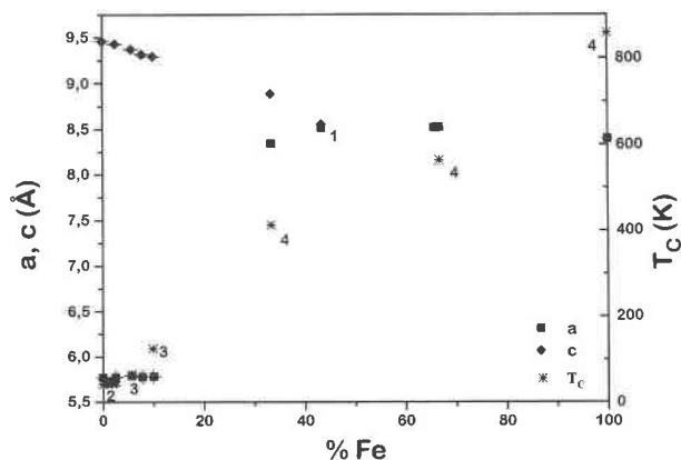
FIGURE 4. Variation of the unit-cell parameters and T_C as a function of the Fe content in \text{Fe,Mn}_{3-x}\text{O}_4 (1 = Evans et al. 1988; 2 = Chardon 1986; 3 = H. Mazaki and S. Tochihiro, personal communication; 4 = Gutzmer et al. 1995).
