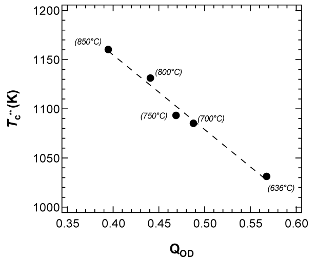
FIGURE 8. Variation of critical temperature, T_c^* , with degree of non-convergent order, Q_{OD} , as extracted from the data for crystal no. 17 in Figure 7. The dashed line is a least-squares fit to the data: T_c^* = 1456(28) - 759(58) \cdot Q_{OD} .
