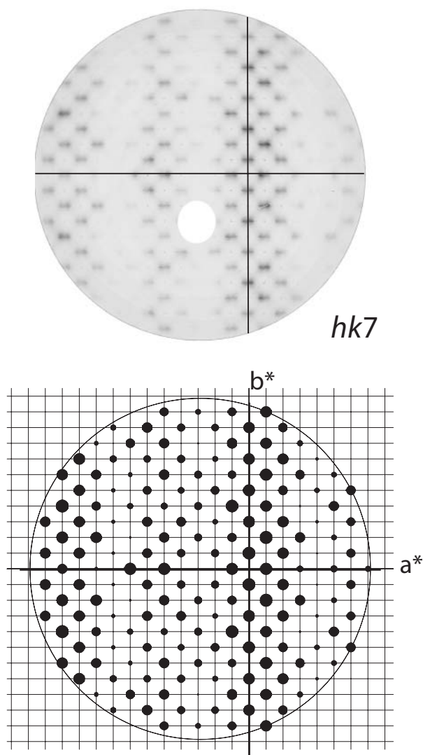
FIGURE 4. Observation and interpretation of the reconstructed hk7 reciprocal space layer of crystal A2. Compare with Figure 3.
