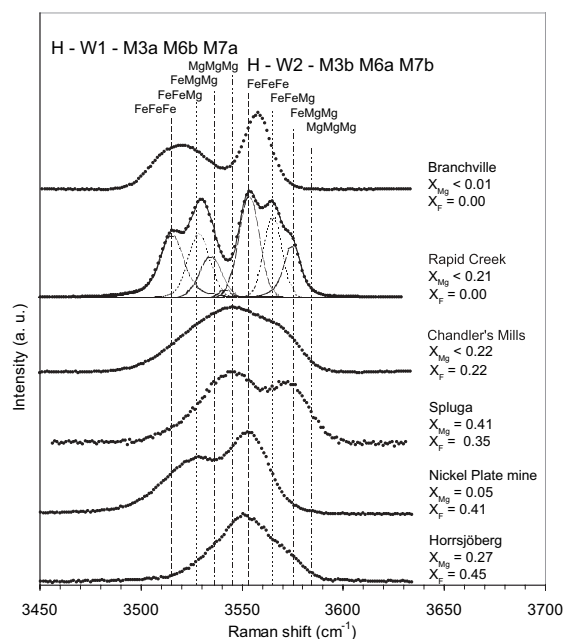
FIGURE 3. Raman spectra (OH-stretching region) of dickinsonite and arrojadite samples arranged in order of increasing fluorine contents. X_F = F/(F + {}^w\text{OH}) , X_{Mg} = Mg/(Mg + Fe + Mn + Zn) . Note the two clusters of bands, which demonstrate that the non-centrosymmetric space group Cc is correct for all the samples. The low-wavenumber cluster is quite weak in Horrsjöberg, suggesting that F is preferentially incorporated at this site. A deconvolution of the Rapid Creek spectrum shows the contribution of various local M3a-M6b-M7a and M3b-M6a-M7b environments around the W1 and W2 sites, respectively.
