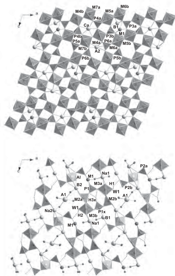
FIGURE 2. Projections onto (010) for the arrojadite structure refined in the Cc space group (this work): (a) the slab at y = 1/4 ; (b) the slab at y = 1/2 .
