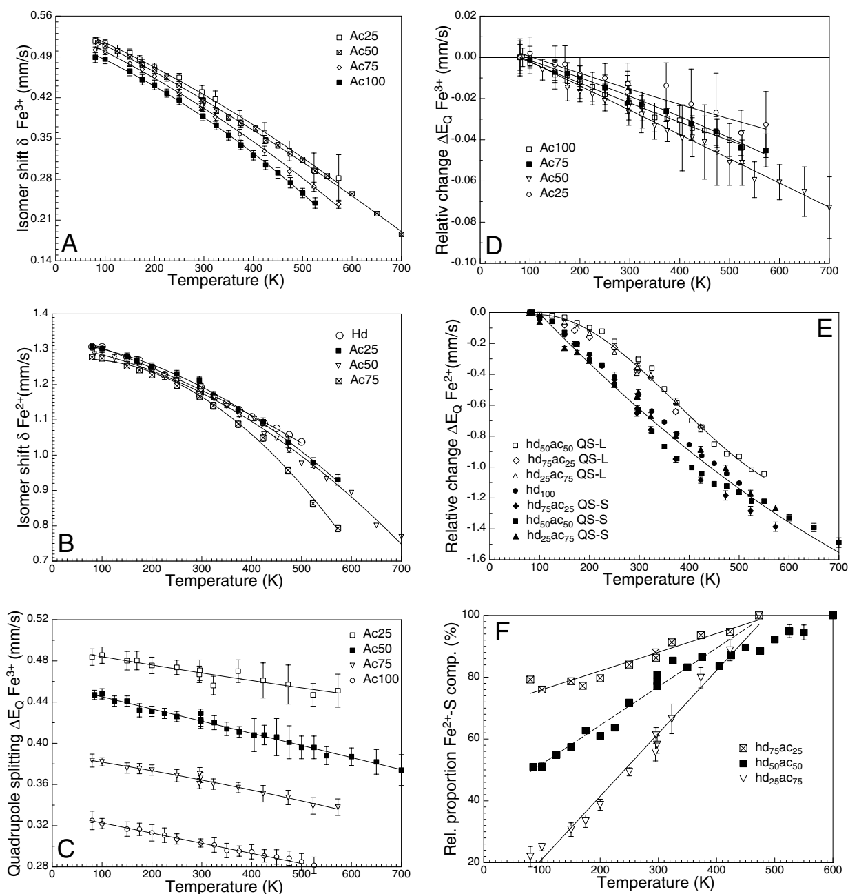
FIGURE 15. Variations of ^{57}\text{Fe} hyperfine parameters of the hedenbergite \text{CaFe}^{2+}\text{Si}_2\text{O}_6 -aegirine \text{NaFe}^{3+}\text{Si}_2\text{O}_6 solid-solution series as a function of temperature: (a) Isomer shift of \text{Fe}^{3+} ; (b) Isomer shift of \text{Fe}^{2+} ; (c) Quadrupole splitting of \text{Fe}^{3+} ; (d) Relative change of \text{Fe}^{3+} quadrupole splitting with respect to the values at 80 K; and (e) Relative change of the \text{Fe}^{2+} quadrupole splitting with respect to the values at 80 K. Lines represent fits to all the data of a group, \text{Fe}^{2+} -L, and \text{Fe}^{2+} -S, respectively.
