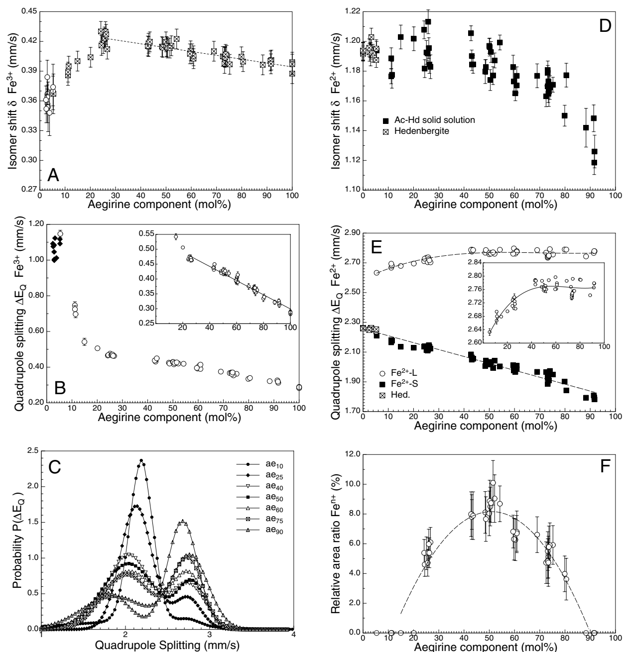
FIGURE 8. Variation of ^{57}\text{Fe} Mössbauer hyperfine parameters within the hedenbergite-aegirine \text{CaFe}^{2+}\text{Si}_2\text{O}_6\text{-NaFe}^{3+}\text{Si}_2\text{O}_6 solid-solution series at 298 K: (a and b) Isomer shift and quadrupole splitting of \text{Fe}^{3+} ; (c) evolution of the \text{Fe}^{2+} quadrupole splitting distribution; (d) isomer shift of \text{Fe}^{2+} ; (e) quadrupole splitting of the two \text{Fe}^{2+} QSD components with the inset showing the variation of the \text{Fe}^{2+}\text{-L} component on an enlarged scale; and (f) relative amount of Fe in the \text{Fe}^{n+} state at 298 K. Error bars are smaller than the symbols if not visible. Lines fitted to the data are guides to the eye.
