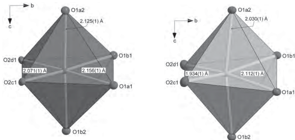
FIGURE 3. Representation of the M1 octahedral geometry viewed along the a -axis at 298 K for (a) hedenbergite- CaFe^{2+}Si_2O_6 , and (b) aegirine- NaFe^{3+}Si_2O_6 .
