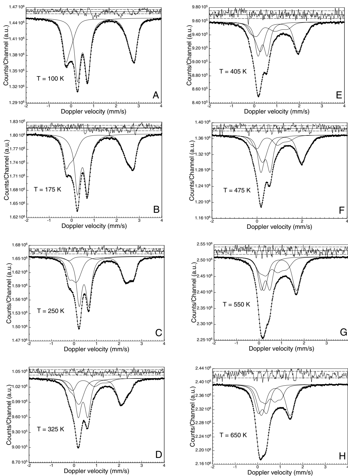
FIGURE 10. Typical ^{57}\text{Fe} Mössbauer spectra of sample Ae5020 ( \text{Hd}_{30}\text{Ae}_{70} ) recorded at different temperatures and evaluated with the quadrupole splitting distribution approach: (a) T = 100\text{ K} ; (b) T = 175\text{ K} ; (c) T = 250\text{ K} ; (d) T = 325\text{ K} ; (e) T = 405\text{ K} ; (f) T = 475\text{ K} ; (g) T = 550\text{ K} ; and (h) T = 650\text{ K} .
