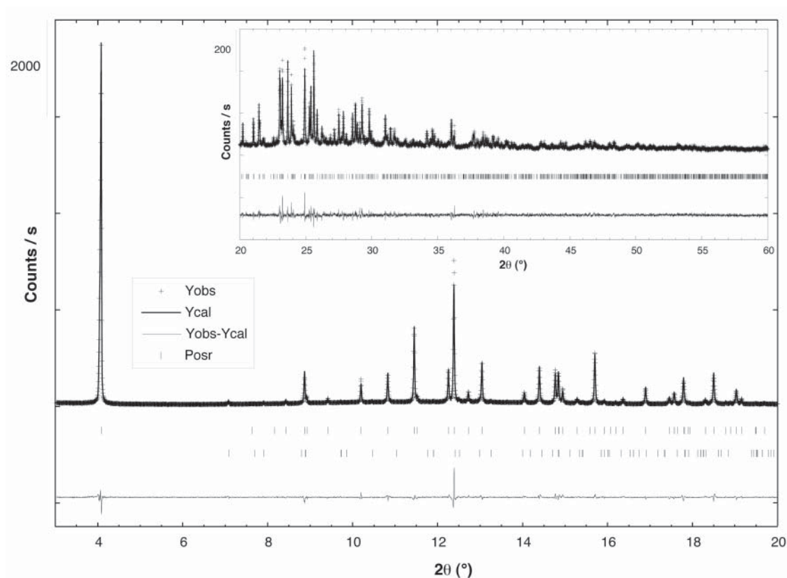
FIGURE 1. Rietveld refinement of the synchrotron XRD powder pattern of the Utah tooeleite sample. Yobs, Ycal, and Yobs-Ycal = experimental, calculated, and difference pattern, respectively. Posr = positions for tooeleite (98 wt%) and scorodite (2 wt%). Detail of the high angle region (20–60° 2 \theta ) is displayed in the inset.
