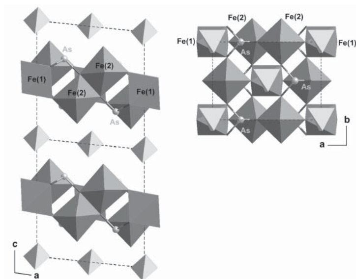
FIGURE 2. The crystal structure of tooeleite, viewed down the [010] and the [001] directions, on the left and right, respectively. The layers are composed of corner and edge sharing \text{FeO}_6 octahedra linked by corners and edges to \text{AsO}_3 pyramids. Isolated sulfate tetrahedra occupy the interlayer space. Only one possible orientation of the sulfate groups with respect to the (010) mirror is represented. In addition, whatever the orientation, only one half of the represented sulfate site is occupied.
