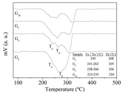
FIGURE 4. DTA traces of the particles formed with different values of Co/Fe.
