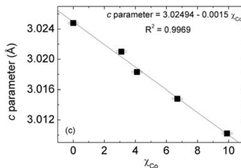
FIGURE 6. Unit-cell parameters vs. Co concentration.
