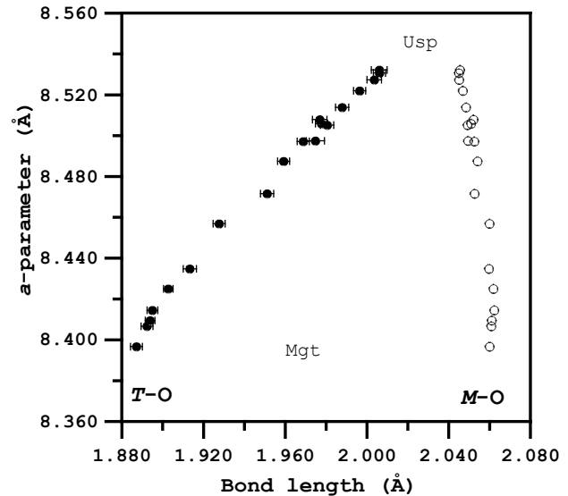
FIGURE 2. The relationships between a -parameter and bond lengths T-O and M-O show that the structure variations are strongly affected by T-O. Symbol dimensions and error bars, where shown, are proportional to 2σ.
