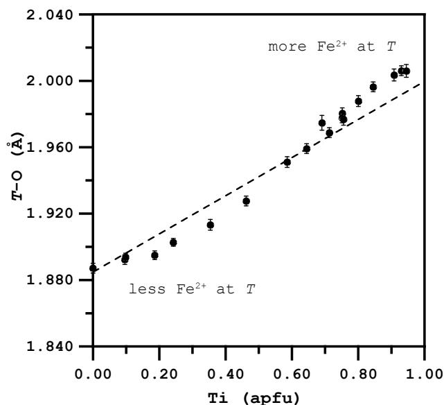
FIGURE 6. Relationship between T-O and Ti, in comparison with the linear variation expected from the Akimoto model (dashed line calculated using empirical bond lengths, see text). ^{\text{T}}\text{Fe}^{2+} contents less than expected yield negative T-O deviations and a region of concave-upward curvature. ^{\text{T}}\text{Fe}^{2+} contents greater than expected yield positive T-O deviations and a region of convex-upward curvature. As a result, the fully occupied site can describe an S-shaped curve. Symbol dimensions and error bars, where shown, are proportional to 2\sigma .
