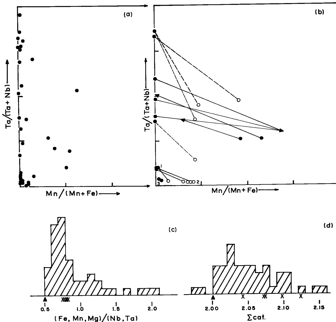
FIG. 2. (a) Bulk compositions of niobian and tantalian rutiles in terms of atomic Ta/(Ta+Nb) and Mn/(Mn+Fe) ratios from the literature; (b) coexisting and exsolved niobian-tantalum rutile + columbite-tantalite pairs in the above plot: 1 niobian rutile and 2 columbite of the Huron Claim symplectite, 3 large grains of the Huron Claim niobian rutile; for other points from the literature, solid dot is the host and arrowhead is the inclusion/exsolution; solid and open circle pairs are coexisting discrete grains of rutile and columbite phases, respectively; (c) frequencies of the (Fe, Mn, Mg)/(Nb, Ta) ratio in niobian and tantalian rutile (at.); triangle denotes the "ideal" value, X marks the Huron Claim ratios; (d) cation totals in niobian and tantalian rutile, based on 4 oxygens (symbols as in c). See text for sources of data.
