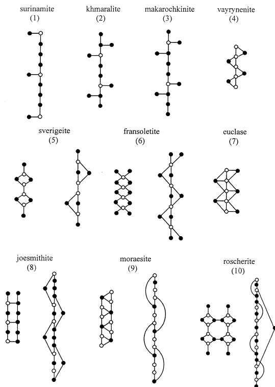
FIG. 5. Graphical representation of (\text{Be}\varphi_4) – (T\varphi_4) chains in Be-bearing minerals; hollow circles are (\text{Be}\varphi_4) tetrahedra, solid circles are other (T\varphi_4) tetrahedra, and the lines connecting the circles indicate corner-linkage between tetrahedra.
