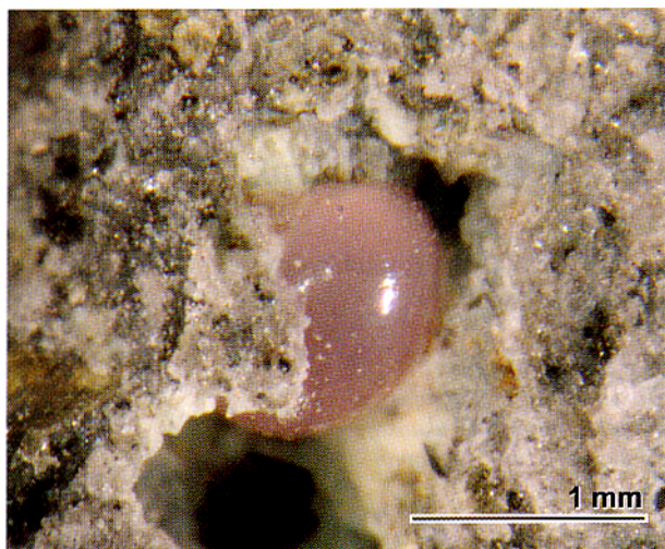
Figure 1 Photomicrographs of the spherical aggregate composed of kozoite-(La) and kozoite-(Nd).
