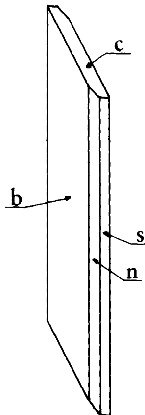
Fig. 2. Typical habit of a coquandite crystal from Pereta. Forms are: b {010}, c {001}, s {210}, n {1, \bar{1} , 2, 0}.
