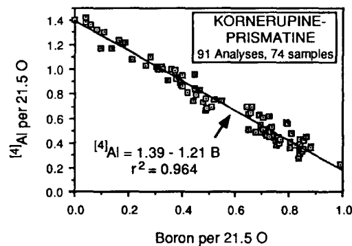
FIG. 1. Plot of 91 kornerupine (here sensu stricto ) and prismatine compositions obtained on 74 samples in terms of boron and ^{141}Al (calculated from 5 - Si - B - Be) per formula unit of 21.5 oxygens. Sources of data are Table 2; Grew et al. (1987, 1990); Friend, 1995; Cooper and Hawthorne, unpublished data; and the literature cited in Grew (in prep.).
