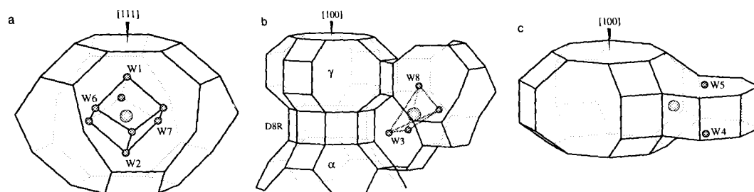
FIG. 5. (a) The cation site M1 (Ca) surrounded by water molecules inside the tetrahedral framework of the \pi -cage; (b) the cation of the M2 site (Ba) surrounded by a tetrahedron of water molecules plus six additional bondings to framework oxygens; (c) the cation site M3 (K) in the centre of the nonplanar 8-ring of the \gamma -cage and the two water molecules in the semicircular band of the five 4-rings attached to the \gamma -cage. The tetrahedral framework is indicated by solid lines representing the T–T bonds, the cations are shown as big (light grey), the water molecules as small (dark grey) balls, respectively.
