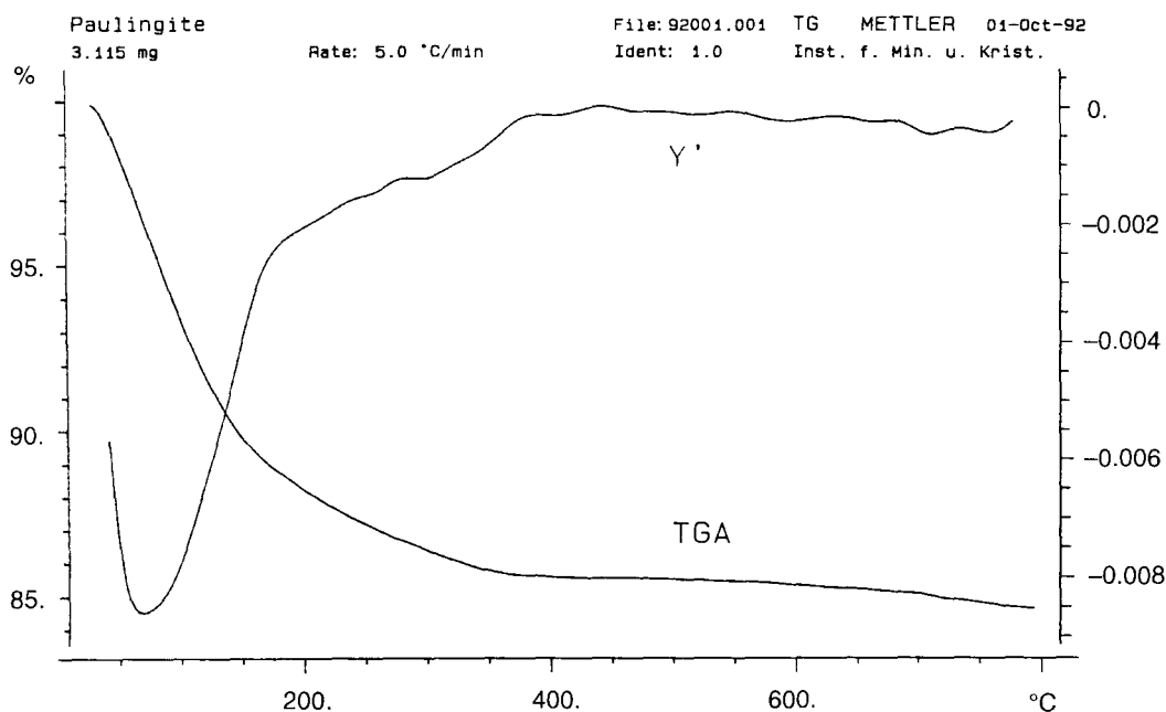
FIG. 2. The thermogravimetric analysis (5°C min -1 ) of paulingite from the Vinarická Hora with weight loss (TG) in wt.% (left axis) and its derivative (Y') in wt.% min -1 (right axis).
