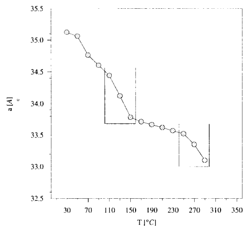
FIG. 4. The cell parameter evaluation of paulingite derived from the Guinier HT-measurement using the 2 \theta values of the (765), (864), and (972) reflections. The error of each data point is \pm 0.1 Å and \pm 5^\circ\text{C} . The boxes indicate the temperature ranges with peak broadening.
