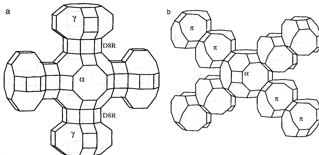
FIG. 1. Three-dimensional slices (a) of the -\gamma -D8R- \alpha -D8R- \gamma - main channel system parallel the plane (\frac{1}{2}, 0, 0) with the dynamic diameter of \sim 4.26 Å, and (b) of the -\pi - \pi - \alpha - \pi - \pi - minor diagonal channel system parallel the plane (110) with the dynamic diameter of \sim 2.50 Å. The \pi -cage can be derived from the levyn-cage with a replacement of the 6-ring plus the neighbouring 4-ring by a single 8-ring.
