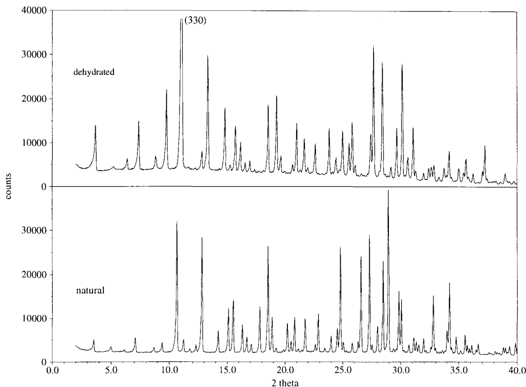
FIG. 3. The observed powder diffraction patterns of the untreated paulingite from the Vinarická Hora and the dehydrated sample. For a better comparison, the (330) reflection of the dehydrated paulingite is clipped at a third of its measured intensity.
