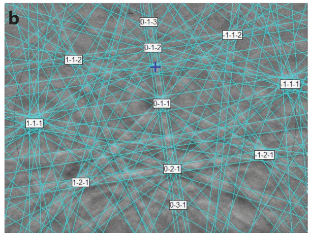
FIGURE 6. (a) EBSD pattern of the adrianite crystal in Figure 2, and (b) the pattern indexed with the \bar{4}3d wadalite structure. (Color online.)
