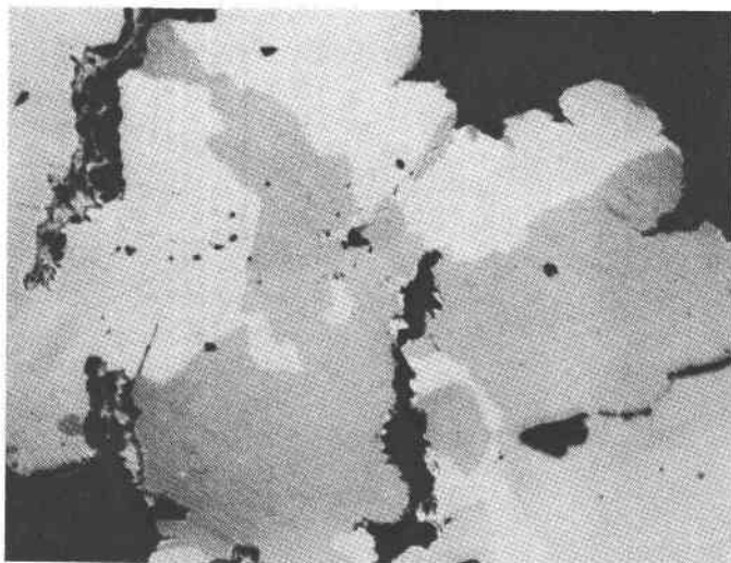
Fig. 1 Polished surface of kutinaite (grey) intergrown with novákite (white) and calcite (black). A sordid of löllingite occurs along the boundaries between calcite and both kutinaite and novákite. 150x.
