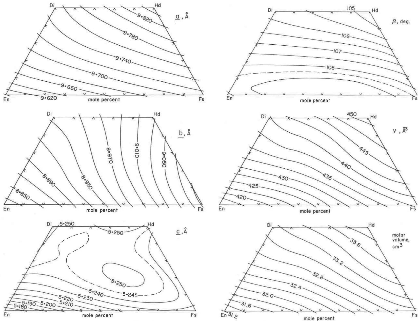
FIG. 2. Contours on trend surfaces showing variation of unit-cell parameters for the synthetic Ca-Mg-Fe clinopyroxenes in Figure 1. Trend surfaces for a , b , c , and \beta are third order; those for V and molar volume are fourth order. Contour intervals are: a , 0.02 Å; b , 0.02 Å; c , 0.01 Å (but note the extra contour for 5.245 Å shown as a dashed line); \beta , 0.5° (but note the extra contour for 108.25° shown as a dashed line); V , 2.5 Å 3 ; molar volume, 0.2 cm 3 /mole, based on z = 8 RSiO 3 per unit cell.
