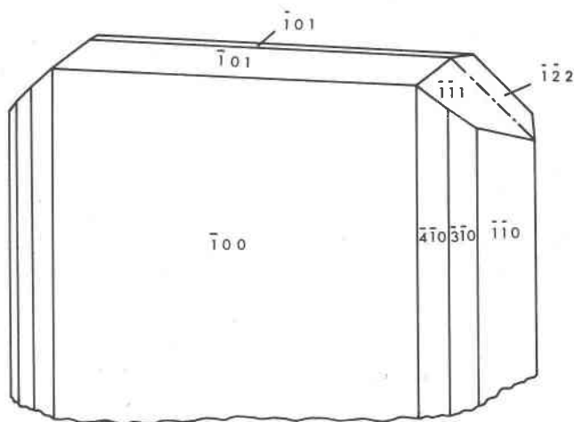
Fig. 1. A simple twin of parascholzite from Hagendorf. The front individual is three times larger than the rear individual. The face g ( \bar{1}11 ) of the front individual continues in the rear crystal as the face f ( \bar{1}22 ) (see text).
