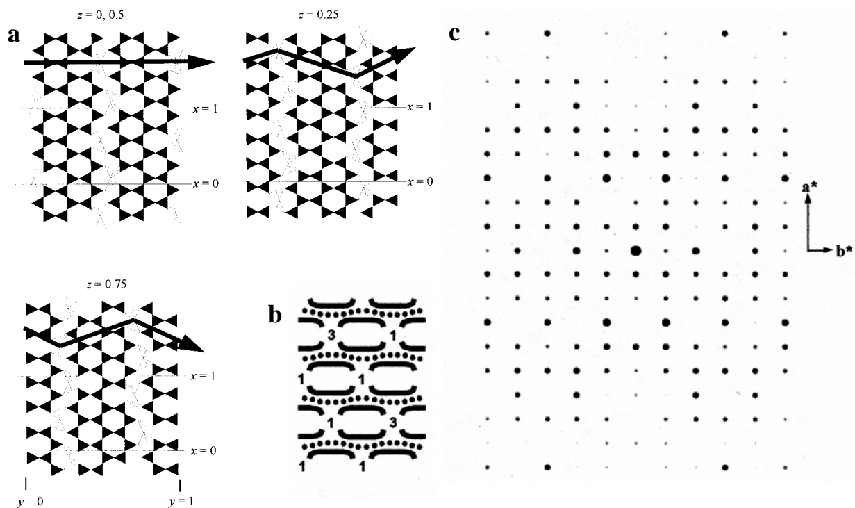
FIGURE 5. Four-layer commensurate cell (type 2). (a) [100] view of tetrahedral strips (not to scale). (b) [100] view of cell (not to scale). (c) Simulated [hk0] diffraction pattern of this structure.
