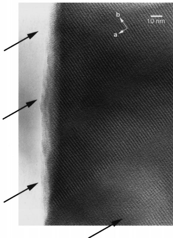
FIGURE 12. Bands of modulation that extend parallel to a (marked by arrows).
