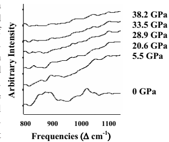
FIGURE 4. Raman spectra of scheelite-structured HfSiO 4 upon release of pressure to room conditions. The transformation of hafnon to a scheelite-structured HfSiO 4 type is quenchable. The inset shows that the high-frequency SiO 4 internal modes of the scheelite-structured HfSiO 4 are not resolved until pressures below 5.5 GPa are reached.
