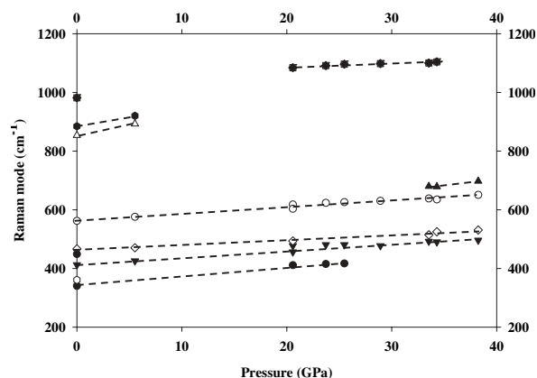
FIGURE 5. Pressure shifts of the vibrational frequencies of scheelite-structured HfSiO 4 obtained on compression and decompression. The high-frequency SiO 4 internal modes of the scheelite-structured HfSiO 4 are not resolved until pressures below 5.5 GPa are reached.
