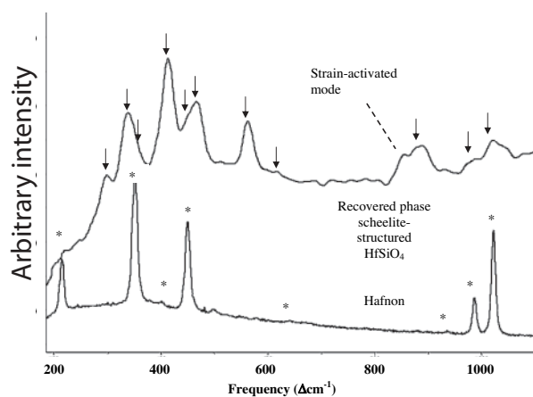
FIGURE 1. Ambient-pressure Raman spectra for \text{HfSiO}_4 (hafnon structure = *) starting material and for the sample quenched from 38.2 GPa and 300 K, which has converted to the scheelite-structured \text{HfSiO}_4 phase (arrows). Peak assignments for the two spectra are given in Tables 1 and 2. The high-pressure resulting spectrum is clearly distinct from the spectrum obtained from the hafnon (starting material) and similar to the reidite spectrum decompressed from the zircon phase transformation.
