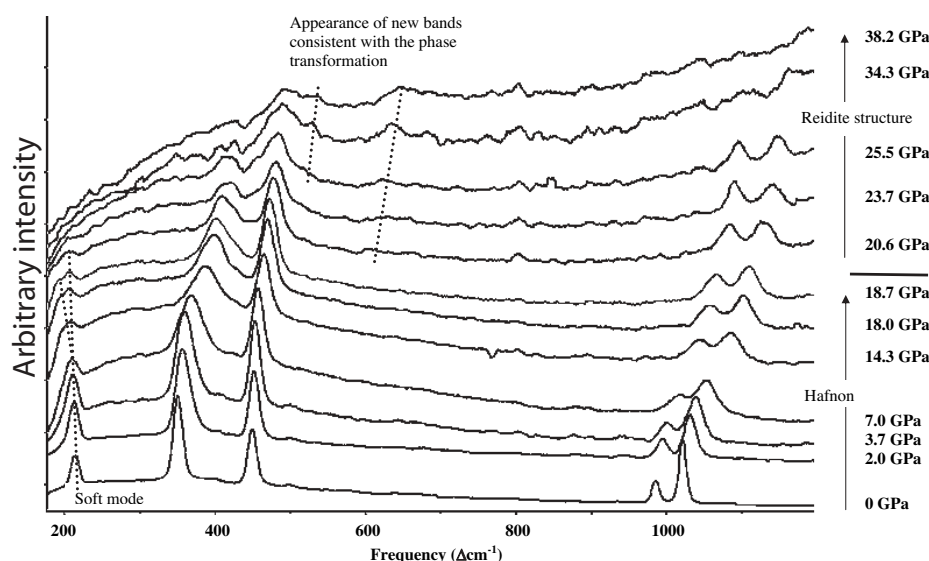
FIGURE 2. Raman spectra through the phase transition from hafnon to scheelite-structured \text{HfSiO}_4 . The spectrum at 20.6 GPa shows the first appearance of a vibration of the scheelite-structured phase at 618\text{ cm}^{-1} , and the spectrum at 25.5 GPa shows the appearance of a second peak in the scheelite-structured phase at 525\text{ cm}^{-1} . The peak observed at 214\text{ cm}^{-1} (1 atm) became undetectable and the 351.3\text{ cm}^{-1} peak disappeared after 25.5 GPa.
