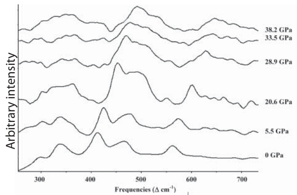
FIGURE 4. Raman spectra of scheelite-structured HfSiO 4 upon release of pressure to room conditions. The transformation of hafnon to a scheelite-structured HfSiO 4 type is quenchable. The inset shows that the high-frequency SiO 4 internal modes of the scheelite-structured HfSiO 4 are not resolved until pressures below 5.5 GPa are reached.
