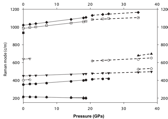
FIGURE 3. Raman frequencies of HfSiO 4 as a function of pressure. Up to 18.7 GPa, HfSiO 4 has the hafnon structure. The appearance of a new vibrational mode at 618 cm -1 at the pressure of 20.6 GPa indicates that the transition to scheelite-structured hafnon has occurred.
