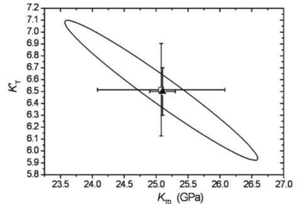
FIGURE 3. Confidence ellipse at the 68.3% level ( 1\sigma , \Delta\chi^2 = 2.30 ) in K_{T0} and K_{T1} for the fit of third-order BM-EoS to the triclinic polymorph P - V data. The BM-EoS K_{T0} and K_{T1} (square) and the co-respective parameters calculated with the fe - Fe plot [ Fe_v(0) and K_{T1} , triangle] are shown. Error bars are \pm 1 e.s.d.
