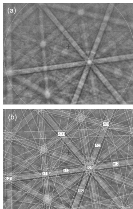
FIGURE 3. (a) EBSD pattern of a murchisite crystal; (b) the pattern indexed with the P\bar{3}1c structure of synthetic Cr 3 S 6 .
