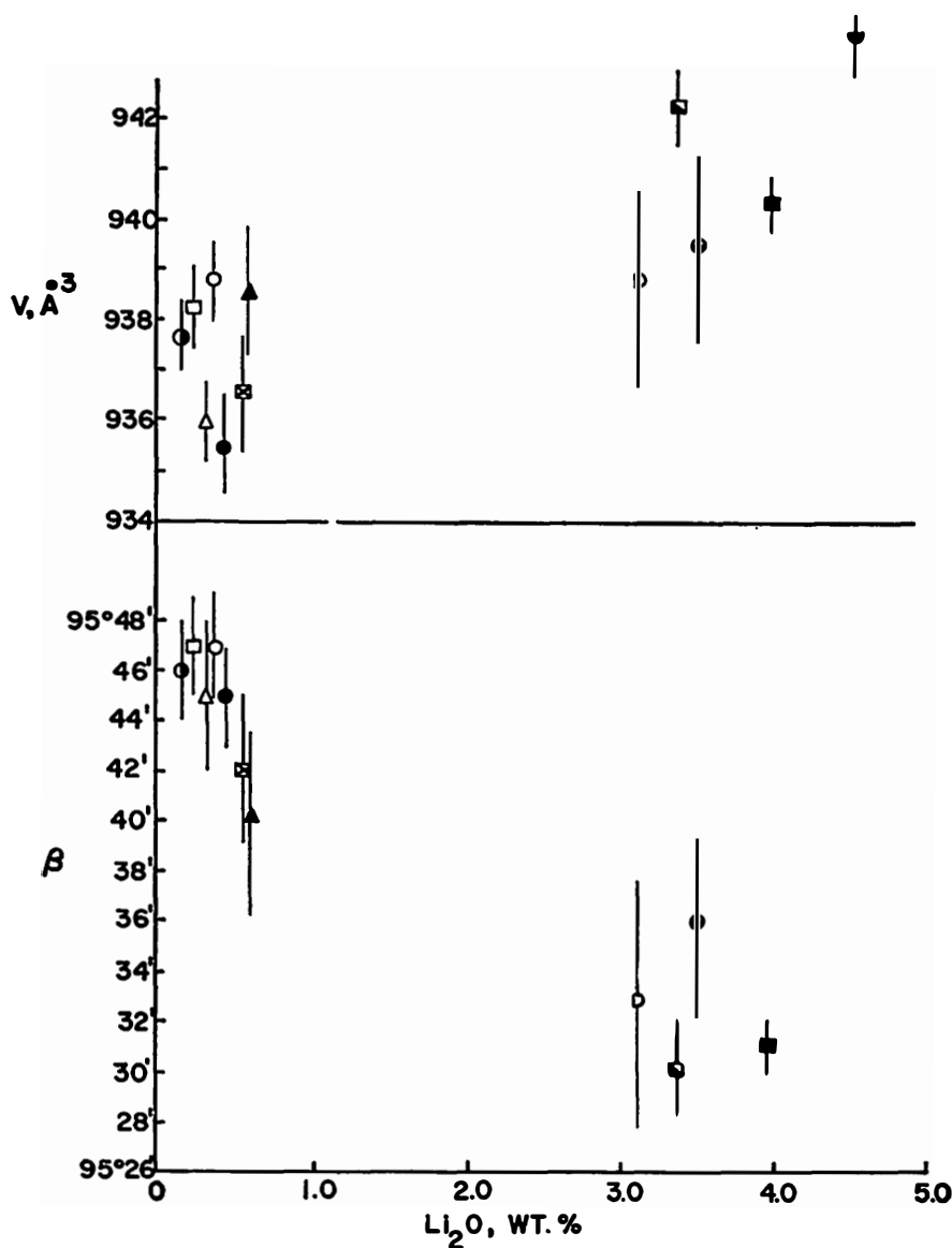
FIG. 5. Variation with \text{Li}_2\text{O} content of the monoclinic angle \beta in 2M_1 structure types, and of the cell volume V in \text{\AA}^3 for all specimens. The specimen numbers corresponding to the different symbols are given in the box in Fig. 6.
