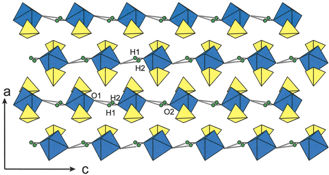
FIG. 3. The crystal structure of orthominasragrite viewed down the b axis; legend as in Figure 1.
