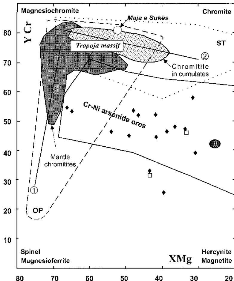
FIG. 6. XMg ( = 100 Mg/\Sigma R^{2+} ) versus YCr ( = 100 Cr/\Sigma R^{3+} ) diagram for chromian spinel hosting anduioite (open square: Kapitanov, open circle: Maja e Sukës). These data are compared with compositions from chromite deposits at Kapitanov (black diamonds), a PGE-rich chromitite from the Tropoja massif (full circle), and with fields for chromite ore from the mantle and cumulate sequence of the Tropoja massif (Neziraj 1992). The two trends (1, 2) illustrate the major substitutions in the mantle and cumulate deposits (see text). The field of Cr-Ni arsenide ores is from Oen et al. (1979) and Gervilla & Leblanc (1990). The field of podiform ophiolitic chromitites (OP) and that of stratiform chromitites (ST) are taken from Gervilla & Leblanc (1990).
