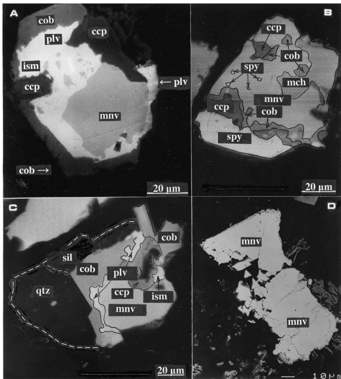
FIG. 3. Textural relationships of menshikovite from the Chiney complex. A. A skeletal crystal of cobaltite [ \text{Co}_{0.72}\text{Ni}_{0.23}\text{Fe}_{0.03}\text{S}_{1.01}\text{As}_{1.02}\text{S}_{1.01} ] contains menshikovite (mnv), paolovite (plv) and isomertieite (ism), which partly replace this menshikovite; note minute relics of menshikovite within the paolovite and isomertieite. ccp is chalcopyrite. B. A complex intergrowth of menshikovite (mnv) with maucherite (mch), sperrylite (spy), cobaltite (cob) and chalcopyrite (ccp). C. An intergrowth of menshikovite (mnv), paolovite (plv), isomertieite (ism), cobaltite (cob), and chalcopyrite (ccp) with quartz (qtz) and a Fe-rich aluminosilicate (sil). D. A large subhedral crystal of menshikovite (mnv). A-D: back-scattered electron images. The black material (Figs. A-D) is epoxy.
