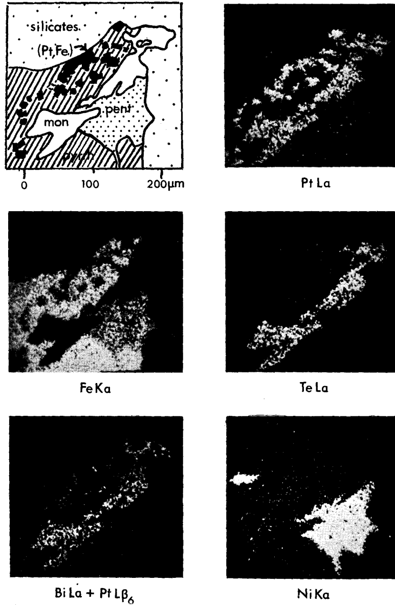
FIG. 2. X-ray scanning micrographs showing the distribution of platinum, iron, tellurium, bismuth, and nickel in an intergrowth of moncheite \text{Pt}(\text{Te}, \text{Bi})_2 (mon) and ferroplatinum (Pt,Fe) in pyrrhotine (pyrrh) and pentlandite (pent) in a polished section of the 'Reef' pyroxenite.
