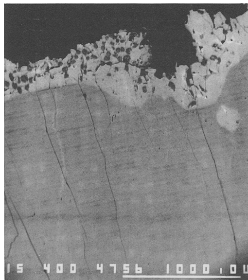
FIG. 1. Back-scattered image of megacryst DZ-19 showing a sanidine core (dark) mantled by hyalophane (bright). Tiny inclusions in the mantle are leucite, Fe-Ti oxides, and glass.
