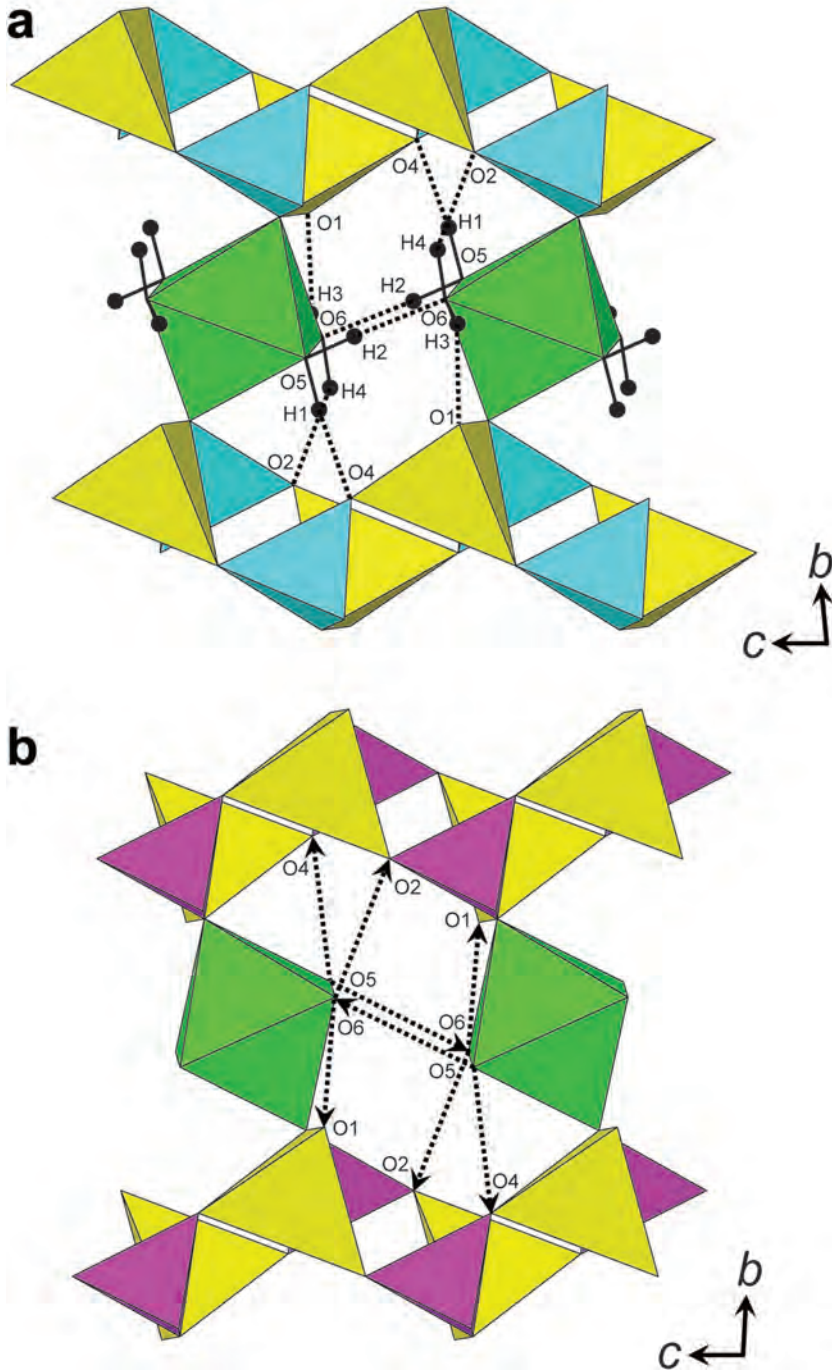
FIG. 5. Hydrogen bonding in (a) davidlloydite and proposed hydrogen-bonding in (b) parahopeite projected down an axis rotated slightly from [100]. The Zn(2)O_4 tetrahedra are yellow, the AsO_4 tetrahedra are blue in davidlloydite and the PO_4 tetrahedra are pink in parahopeite, Zn(1) octahedra are green.
