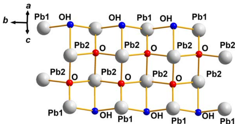
FIG. 4. The [\text{O}(\text{OH})\text{Pb}_2]^+ chains in the crystal structure of yeomanite.
