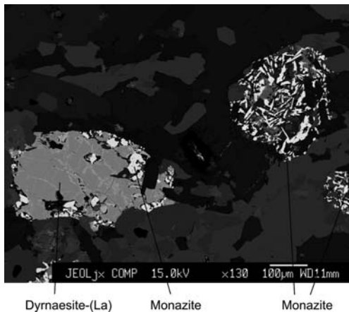
FIG. 3. Back-scattered electron image of dyhaesite-(La) with inclusions of anhedral monazite and two clusters with lath-formed monazite.
