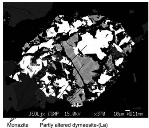
FIG. 4. Back-scattered electron image of altered dyhaesite-(La) with clusters of anhedral monazite.
