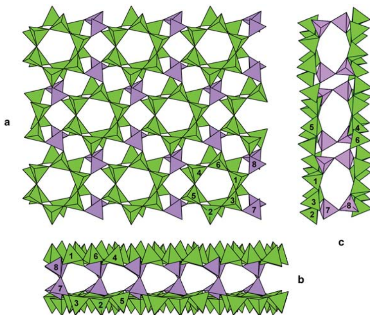
FIG. 3. The double-layer borosilicate sheet in odigitriaite; (a) plan view (viewed in the c direction); (b,c) cross sections. T (1–6) (= Si) tetrahedra: green; T (7–8) (Si,B) tetrahedra: violet. The numbers indicate the different T tetrahedra.
