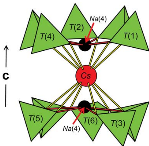
FIG. 2. The Cs and Na(4) sites within the double-layer sheet of odigitriaite; Cs: large red circle; Na(4): small black circle; (\text{SiO}_4)^{4-} tetrahedra: green; Cs–O bonds are indicated by yellow lines. Cs–Na(4) = 2.00 Å, Na(4)–Na(4) = 4.00 Å; hence locally adjacent Cs–Na(4) sites cannot both be occupied, whereas locally adjacent Na(4)–Na(4) sites can both be occupied.
