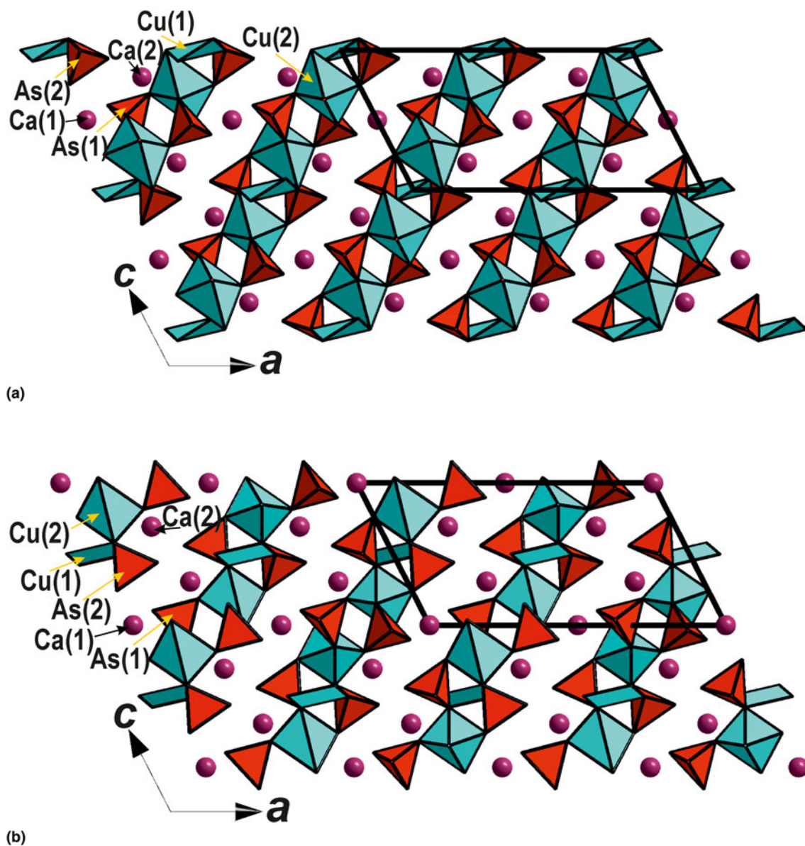
Fig. 6. Crystal structures of zerkovaite (a) and synthetic \text{Ca}_3\text{Cu}_3(\text{AsO}_4)_4 (b, drawn after Osterloh and Müller-Buschbaum, 1994). The unit cells are outlined.
