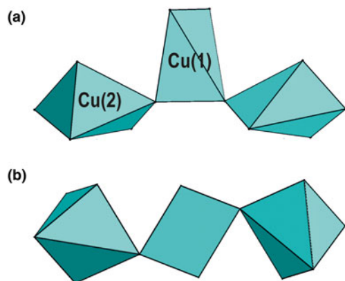
Fig. 7. Trimers of Cu-centred polyhedra in the crystal structures of zerkovaite (a) and synthetic \text{Ca}_3\text{Cu}_3(\text{AsO}_4)_4 (b, drawn after Osterloh and Müller-Buschbaum, 1994).
