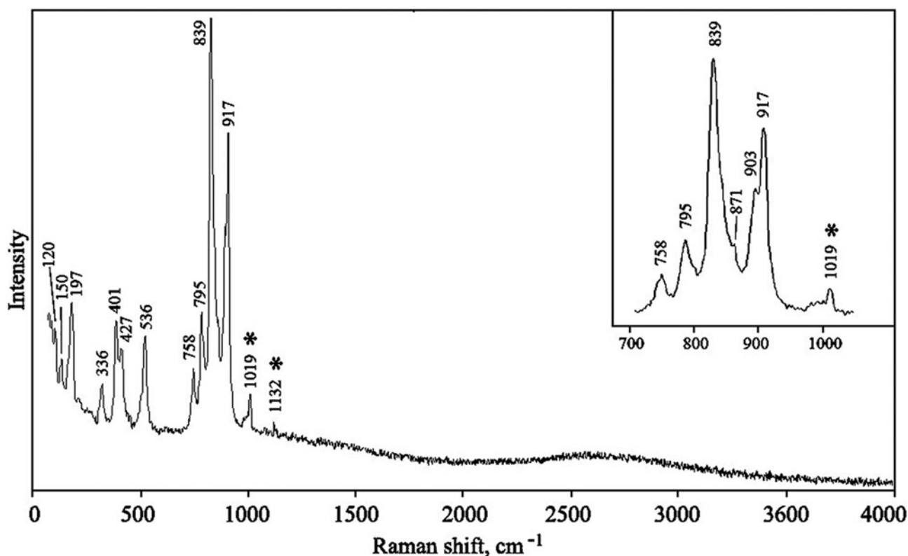
Fig. 5. The Raman spectrum of zuckovaite; bands corresponding to admixed anhydrite are marked with an asterisk.
