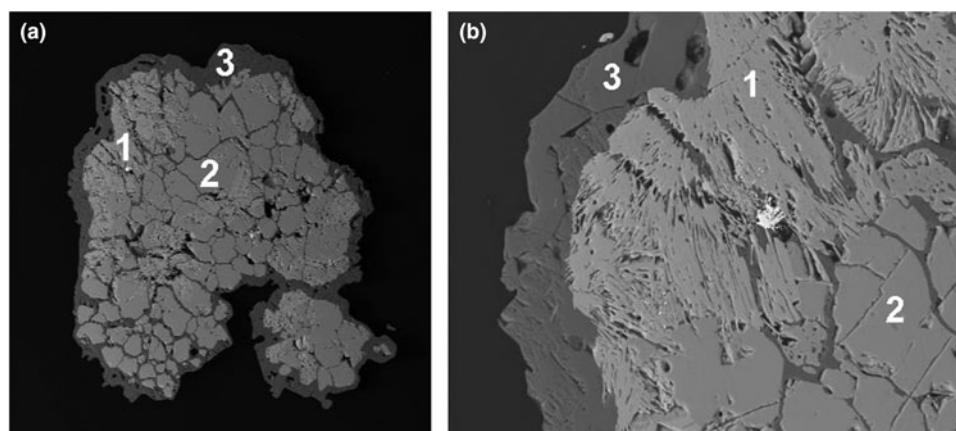
Fig. 3. Clusters of zubkovaite (1) and svabite (2) coated by anhydrite (3); anhydrite crusts (which look like veinlets in the section) are also observed around separate svabite individuals and zubkovaite aggregates: (a) polished cross-section; (b) its magnified fragment. The holotype specimen, catalogue number 96202. SEM back-scattered electron images. Field of view width: (a) 1.5 mm; (b) 0.35 mm.
