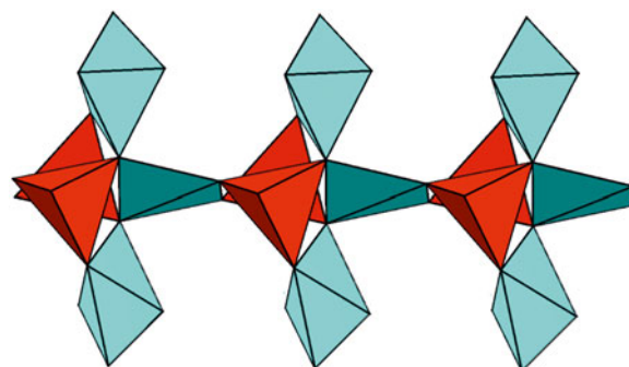
Fig. 8. Ribbon formed by the trimers of Cu-centred polyhedra linked via As(2)O 4 tetrahedra in the crystal structure of zerkovaite. For legend see Fig. 6.
