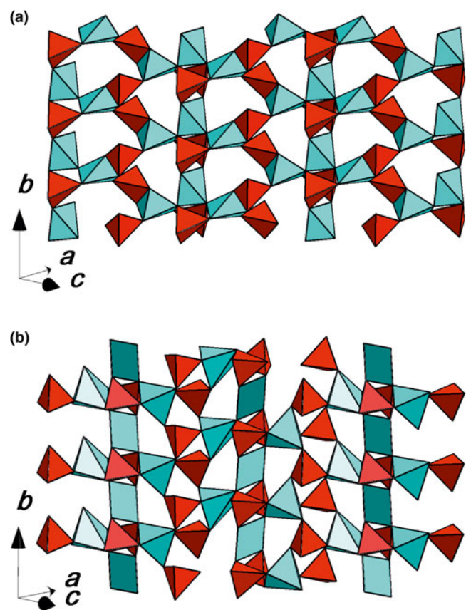
Fig. 9. Heteropolyhedral Cu–As–O layers in the crystal structures of zulkovaite (a) and synthetic Ca 3 Cu 3 (AsO 4 ) 4 (b, drawn after Osterloh and Müller-Buschbaum, 1994). For legend see Fig. 6.
