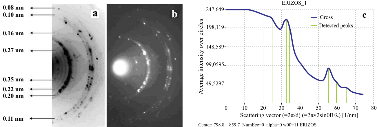
Figure 6. a, b: Selected area electron diffraction (SAED) pattern from many thorns as those shown in Figure 4; (a) shows the inverse contrast from (b) for clarity. This polycrystalline diffraction pattern can be indexed as K_3(VS_4) and as cristobalite. C: SAED intensities profile obtained from process diffraction software package (one region of the sample with the “hedgehog”-like particles).
