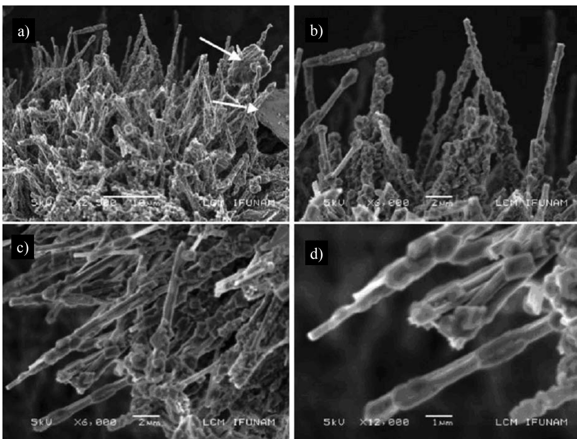
Figure 4. SEM images, taken at 5 kV, of the thorns of a “hedgehog”-like particle. Note the existence of irregular and regular particles among them, such as those shown in (a) and indicated by the arrows. Also note that the thorns are in fact formed by many small and regular particles.
