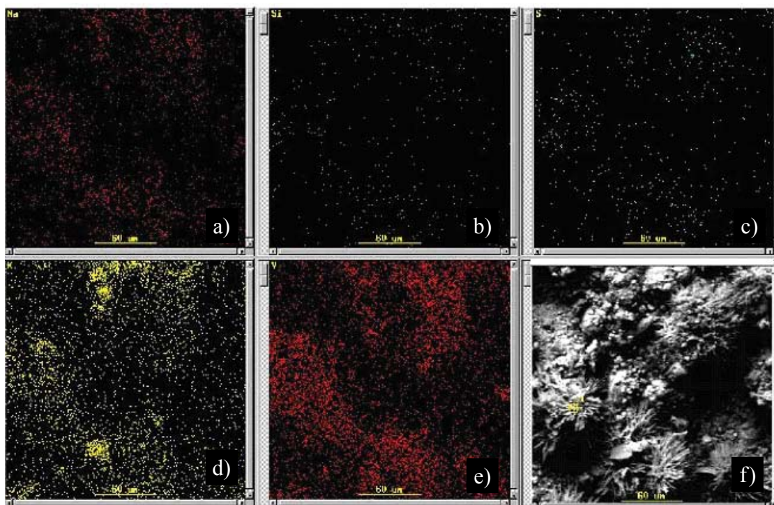
Figure 5. EDS mapping from an area containing both the “hedgehog”-like particles and their environs. a: Na, b: Si, c: S, d: K, e: V, and f: SEM image of the area under observation.
