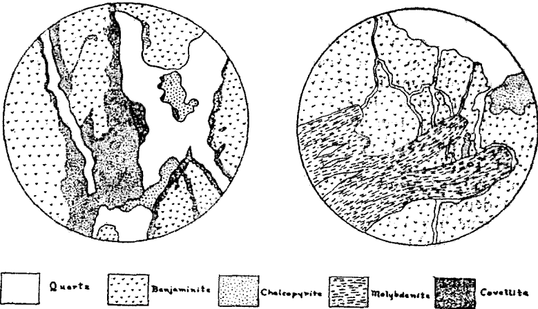
FIG. 1.—SKETCH OF POLISHED SURFACE OF BENJAMINITE SHOWING RELATION OF BENJAMINITE TO QUARTZ AND CHALCOPRYRITE AND REPLACEMENT OF CHALCOPRYRITE AND BENJAMINITE BY COVELLITE. FIG. 2.—SKETCH OF POLISHED SURFACE SHOWING RELATIONS OF BENJAMINITE, MOLYBDENITE, CHALCOPRYRITE, AND QUARTZ.
