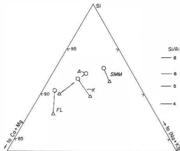
FIG. 4. Si-Ca+Mg-(Na+K 2 ) plot of associated ferrierite (circles) and clinoptililite or heulandite (triangles). Locality symbols are the same as in Figure 1. The points represent averages of all analyses of each mineral from each locality.
