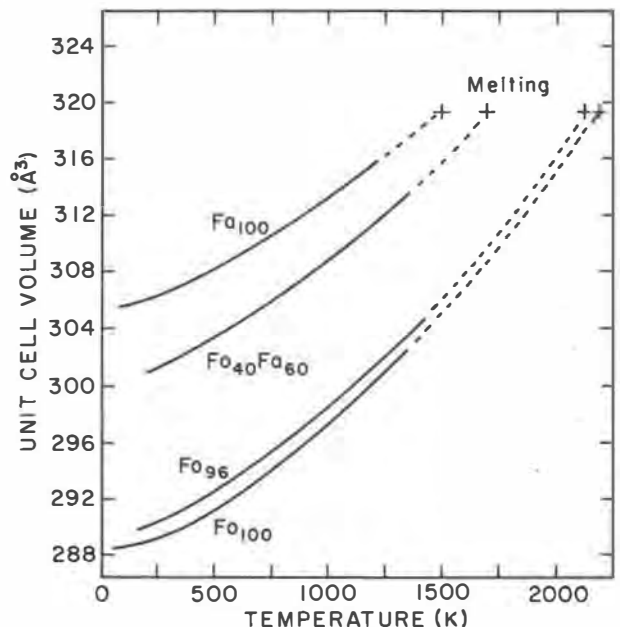
FIG. 2. Olivine unit-cell volume versus temperature. Volumes are calculated from linear expansion data recorded in Fig. 1.
