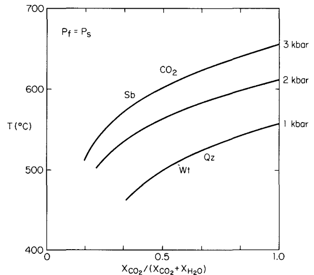
Fig. 1. Calculated decarbonation equilibria for the reaction: Witherite (Wt) + Quartz (Qz) = Sanbornite (Sb) + CO 2 .
