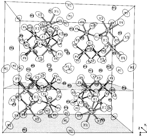
Fig. 1. ORTEP II (Johnson, 1976) drawing of calzirtite showing all metal atoms in the unit cell. The octahedral coordination spheres are also illustrated. Two planes are shaded at y = 0 and y = 1/2 . M1 = Zr; M2 = Ti, Fe, Nb; M3 = Ca; M4 = Zr; X1-X5 = oxygen.
