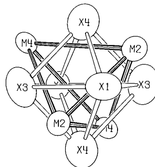
Fig. 4. Illustration of the cation tetrahedron (M2, M4) and anion octahedron (X1, X2, X3, X4) surrounding the vacant anion site at (1/4, 0.5833, 1/2) .
