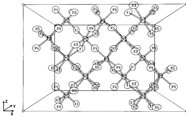
Fig. 2. Diagram of the plane of metal atoms shaded in Fig. 1 at y = 1/2 . The completed coordination spheres of the cations have been included.
