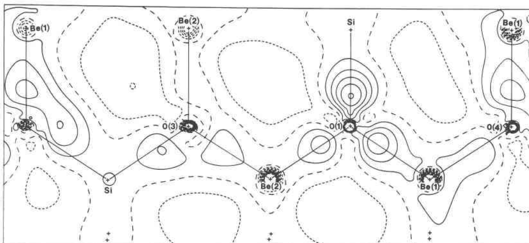
Fig. 3. Static deformation density computed in direct space from a superposition of spherical GSFs and multipole deformation functions. Contour interval 0.1 \text{ e } \text{\AA}^{-3} .
