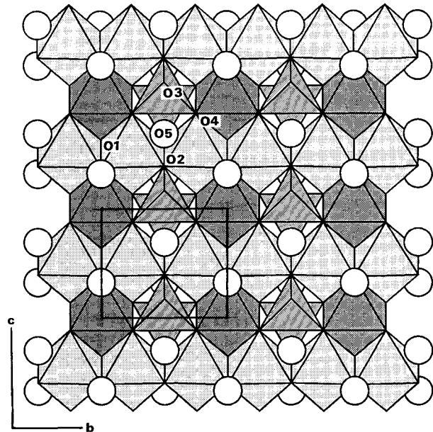
Fig. 2. A projection of the cianciulliite structure on (100). Mn octahedra are darkly shaded, (Mg,Mn) octahedra are lightly shaded, Zn tetrahedra are ruled, and H 2 O molecules (O5) are large open circles. The unit cell is outlined.
