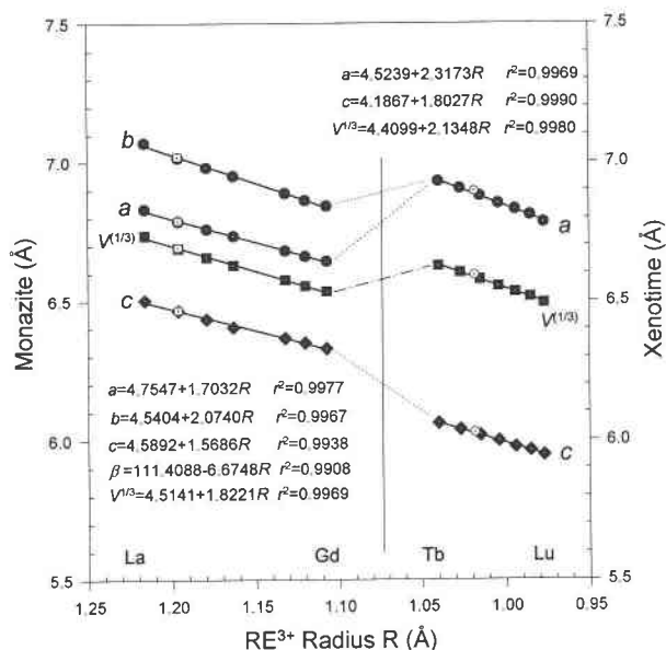
Fig. 1. Variation of lattice parameters with RE element for synthetic RE(PO 4 ) phases. RE radius from Shannon (1976). Open symbols denote natural phases analyzed in this study.
