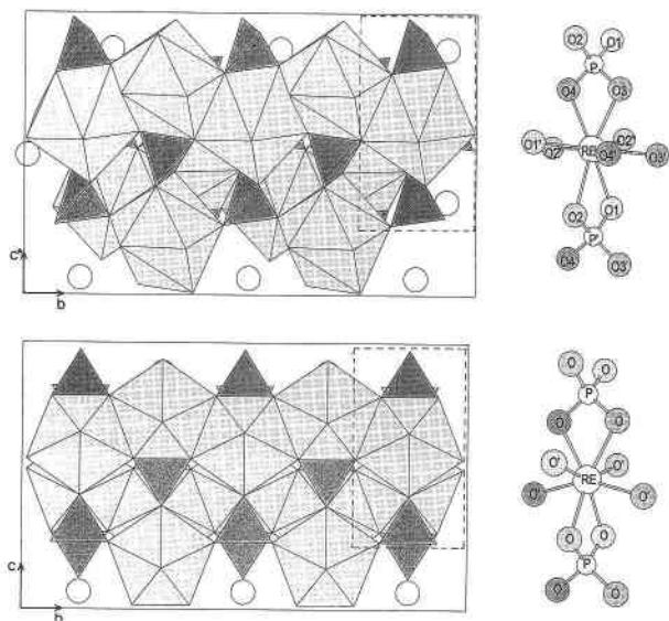
Fig. 2. Atomic arrangements of monazite (top) and xenotime (bottom). Polyhedral projections down [100] illustrate the similarity between the two atomic arrangements. Ball and stick chains and atomic nomenclature for each structure are depicted to right; ball and stick depictions are rotated about c^* for clarity of viewing. Dashed line outlines polyhedron-tetrahedron chain illustrated on right. Open circles represent RE atoms.
